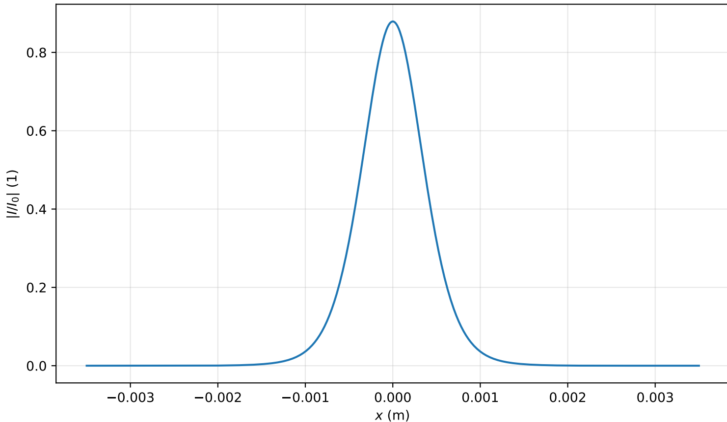
Intensity profile I(x, y = 0, z = 2.229m)/I_0 , P_{in}=0.6P_{cr} , artificial time
